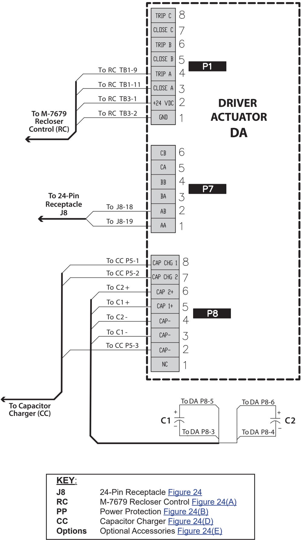
Figure 24(C) Cabinet Interface 24M – Driver Actuator (DA) Connections
