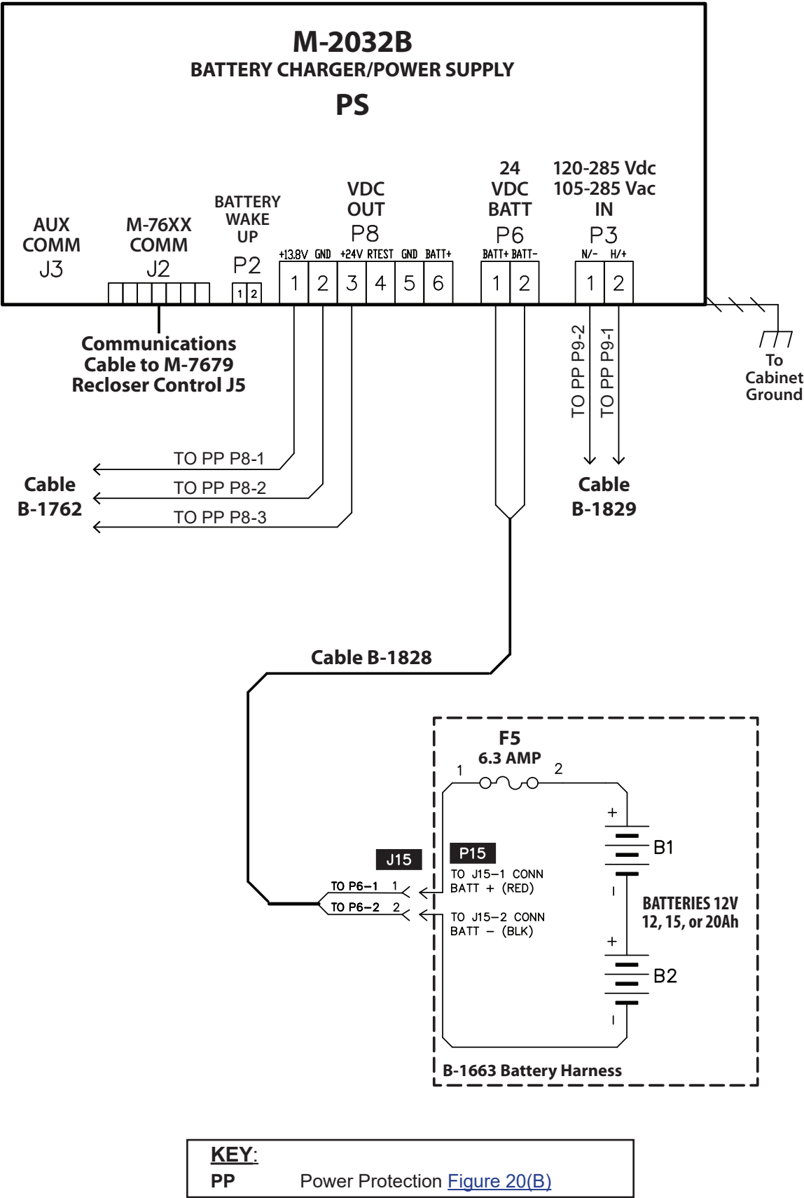
Figure 20(C) Cabinet Interface 14C2, 14G2 – M-2032B Battery Charger/ Power Supply Connections
