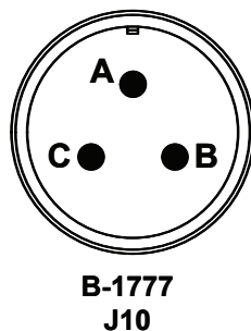
Figure 40 3-Pin Cannon AC Input Cable B-1777
