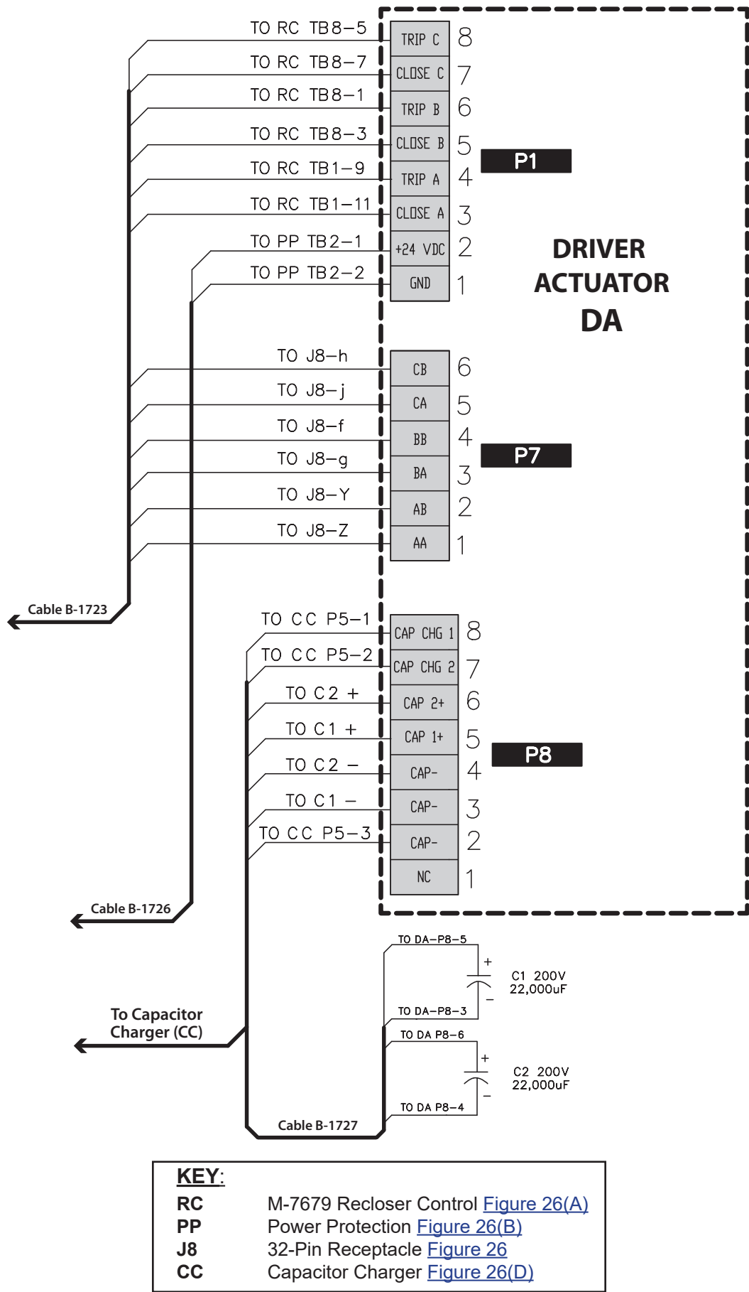
Figure 26(C) Cabinet Interface 32B – Driver Actuator (DA) Connections
