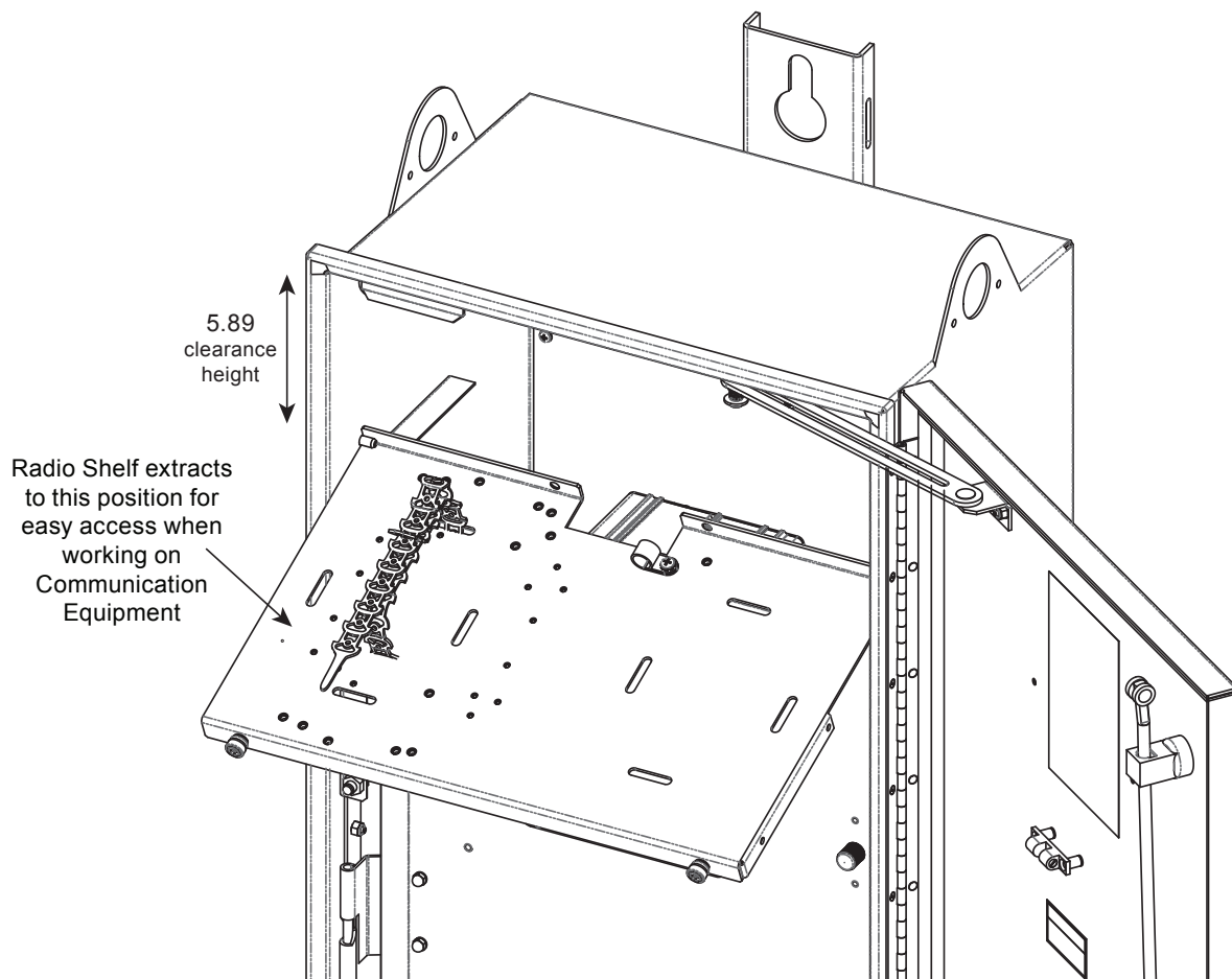
Figure 44 Radio Shelf Extended
