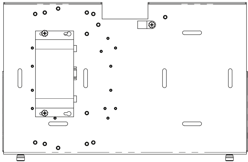
Figure 45 Airlink Raven X or GS & GX Series
