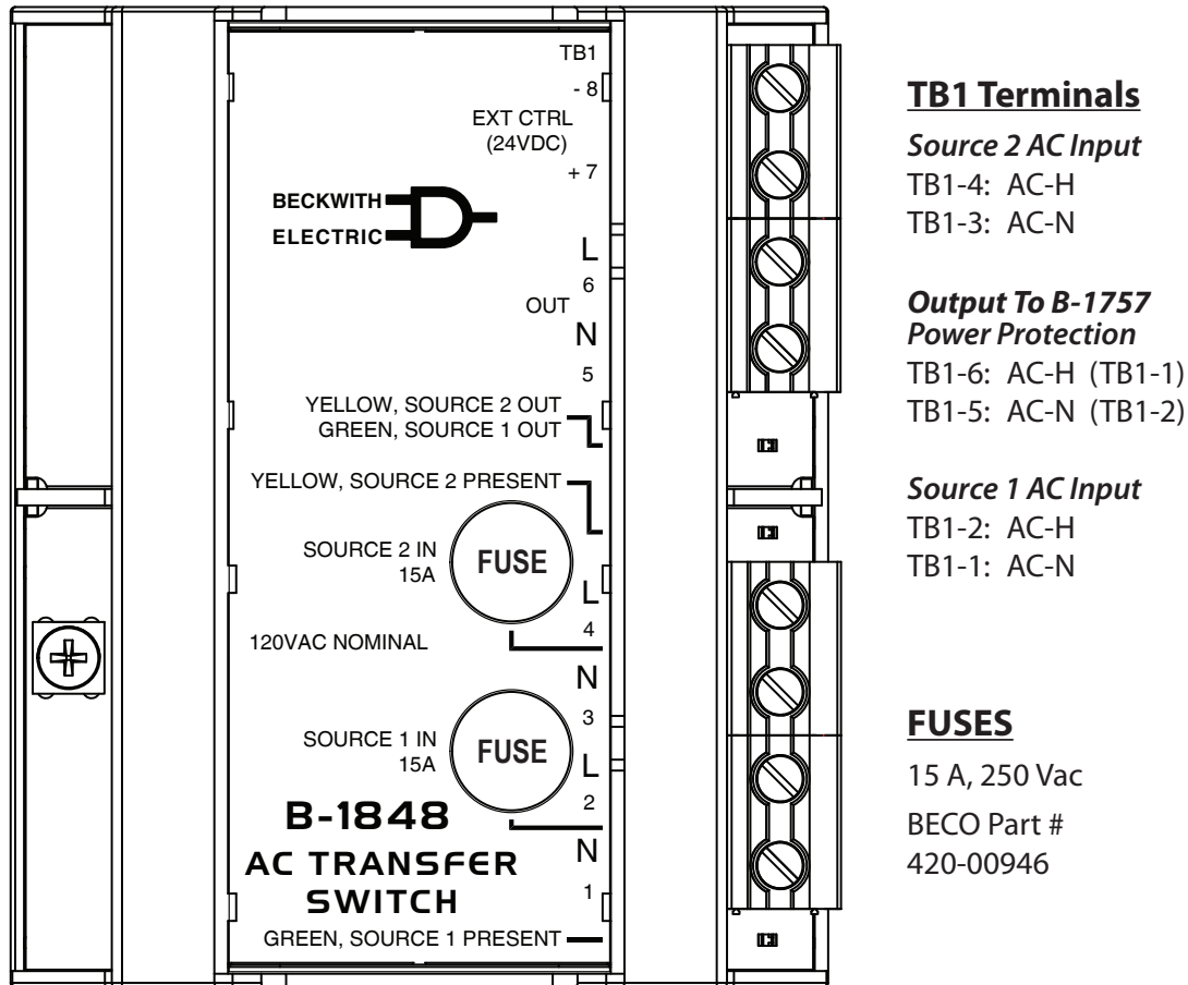
Figure 38 AC Transfer Switch (B-1848)
