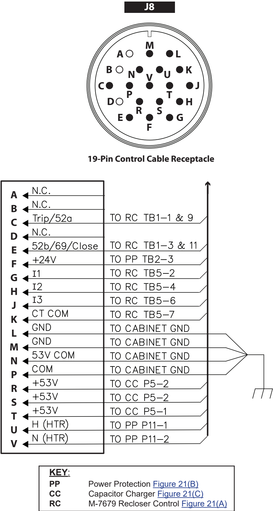
Figure 21 Cabinet Interface 19B – 19 Pin Control Cable Receptacle Pinouts
