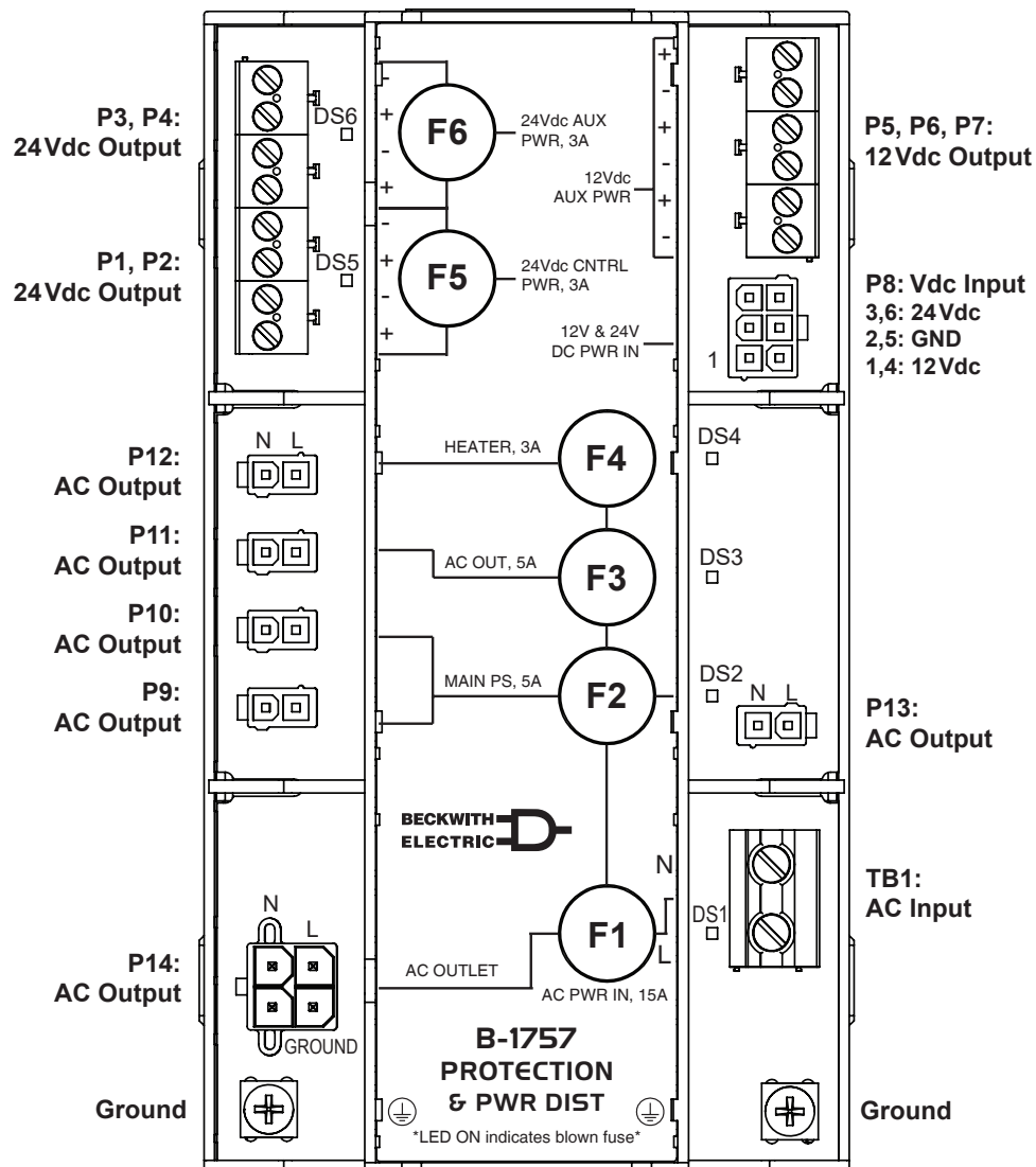
Figure 16 Power Protection & Distribution Module (B-1757)
