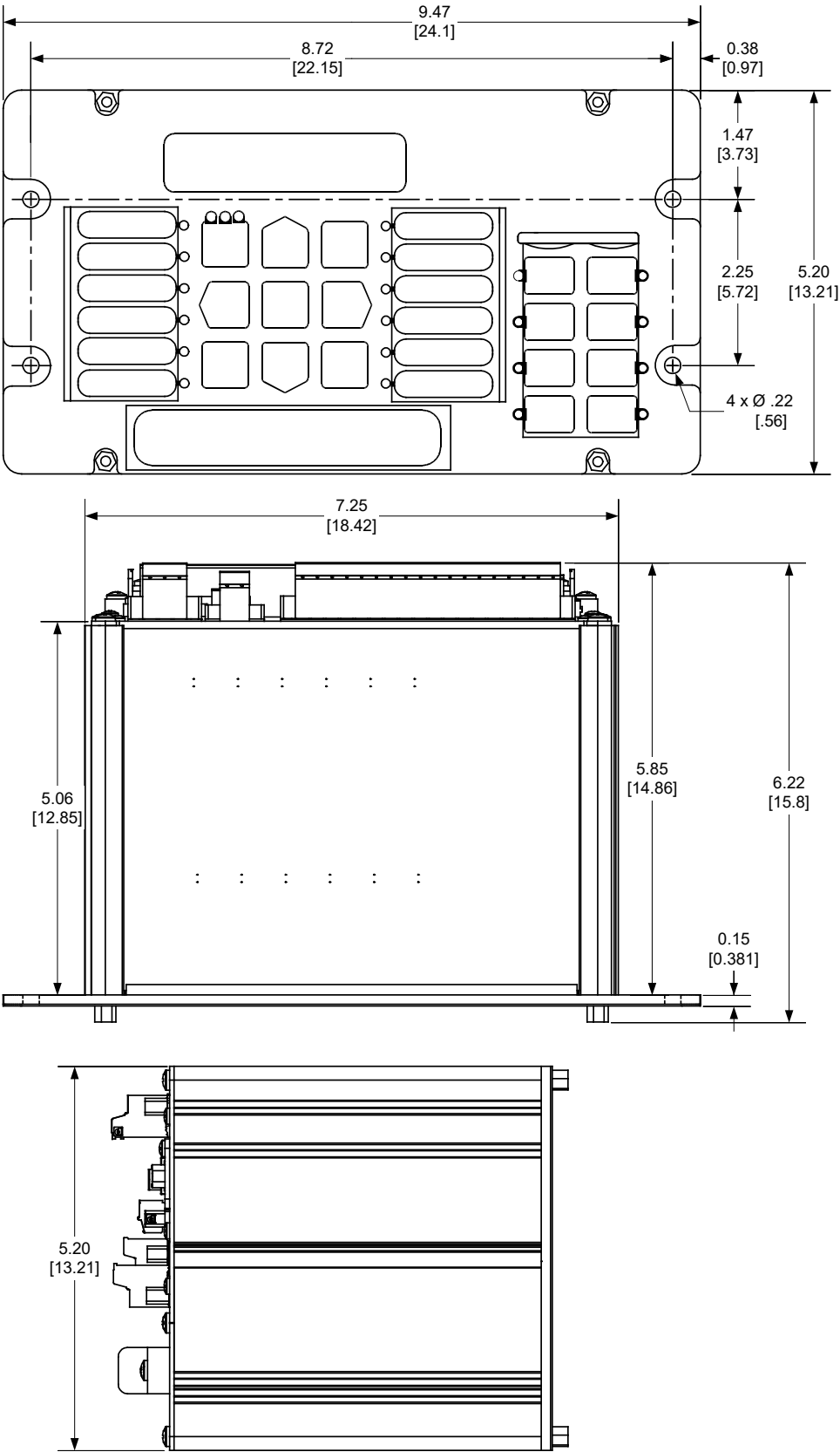
Figure 2 M-7679 Horizontal Model Mounting Dimensions
