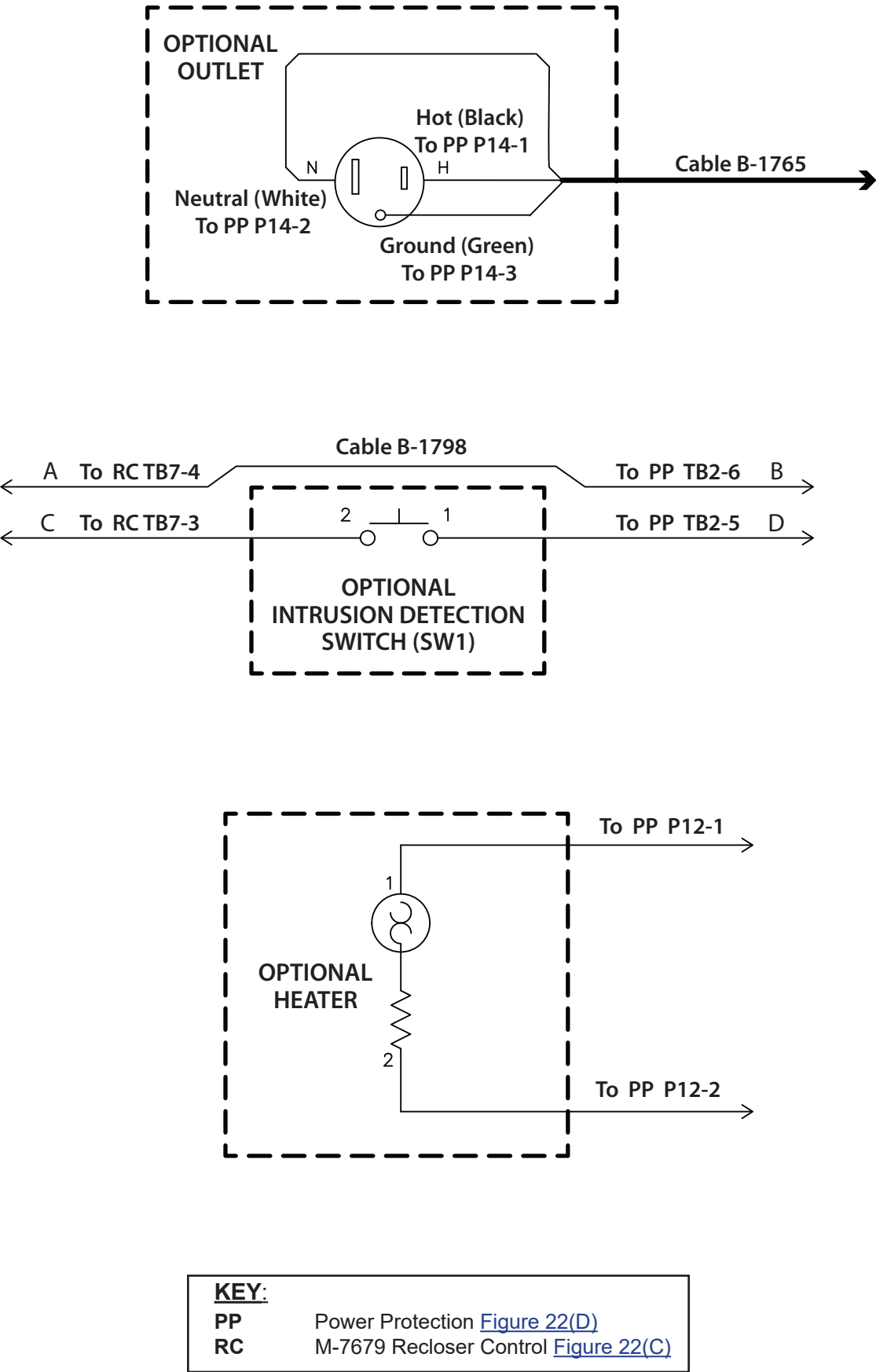
Figure 22(G) Cabinet Interface 24A – Optional Accessories Connections
