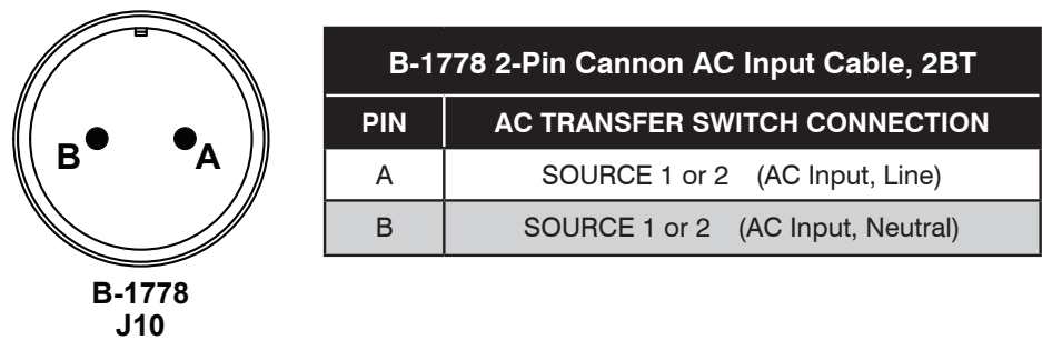
Figure 41 2-Pin Cannon AC Input Cable B-1778
