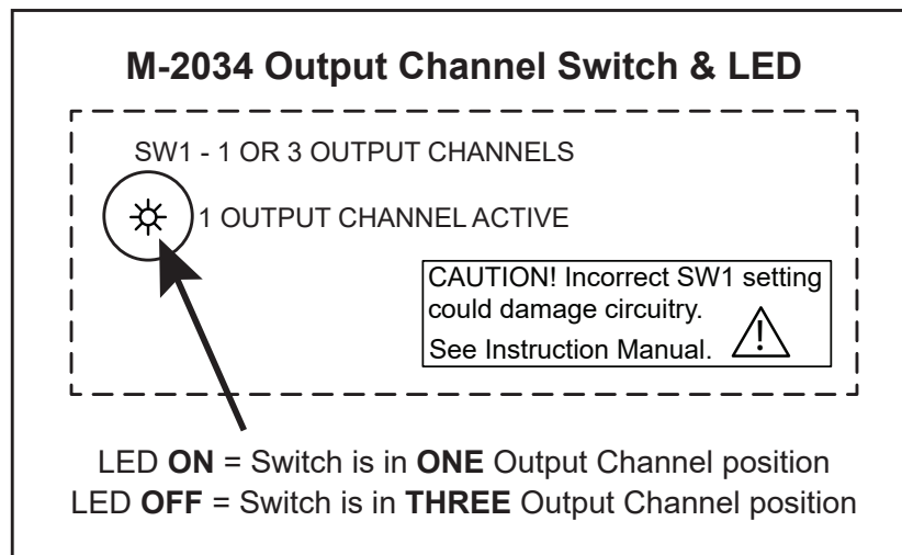
Figure 14 M-2034 Output Channel Switch Position Indicator LED
