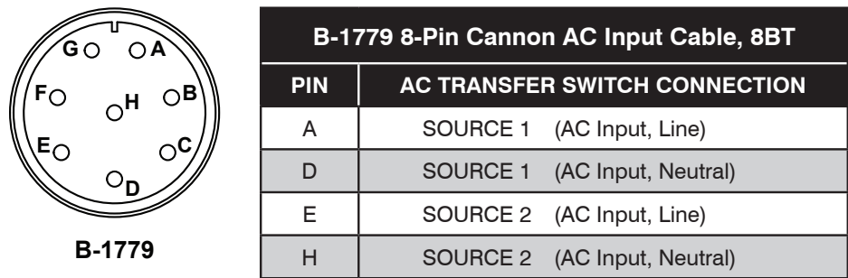
Figure 42 8-Pin Cannon AC Input Cable B-1779
