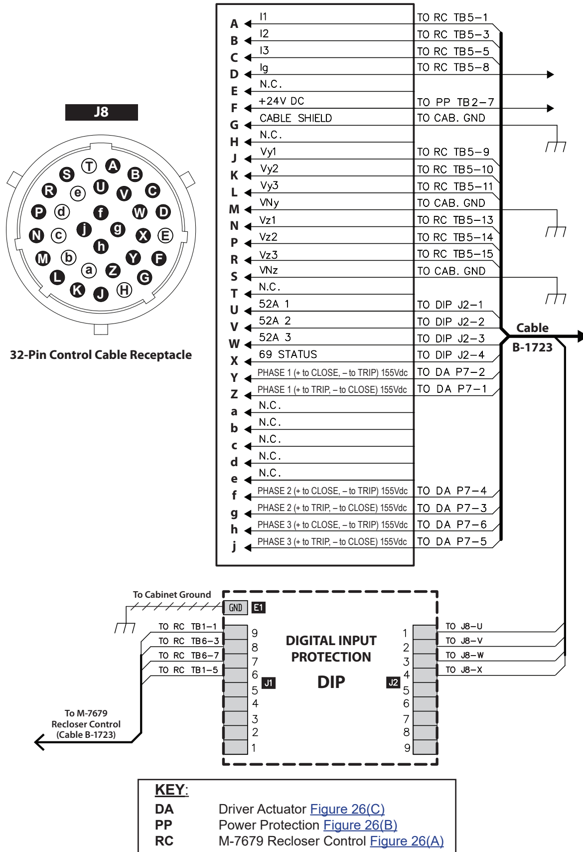
Figure 26 Cabinet Interface 32B – 32 Pin Control Cable Pinouts & DIP Board
