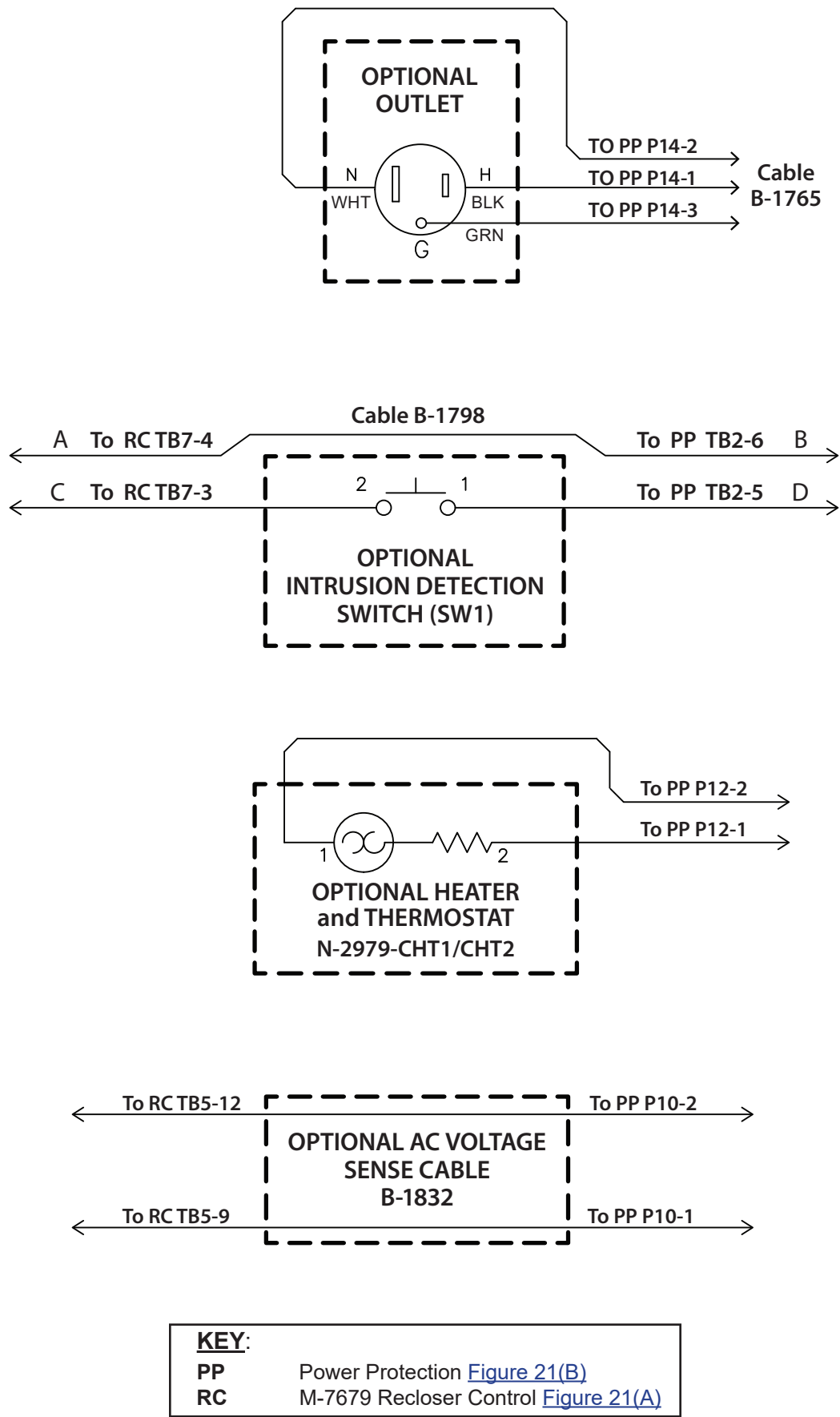
Figure 21(D) Cabinet Interface 19B – Optional Accessories Connections
