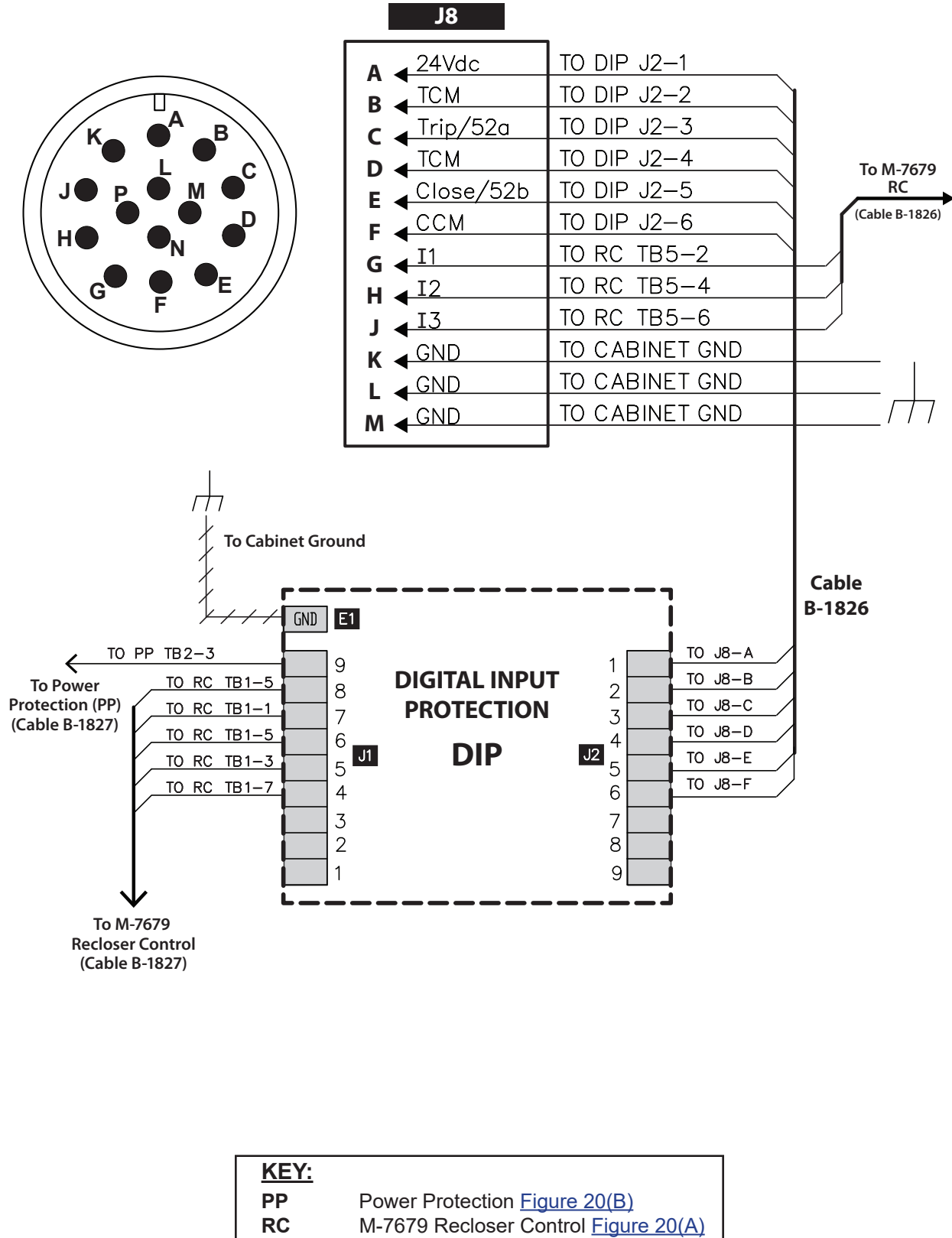
Figure 20 Cabinet Interface 14C2, 14G2 – 14 Pin Control Cable Receptacle Pinouts and Digital Input Protection Board
