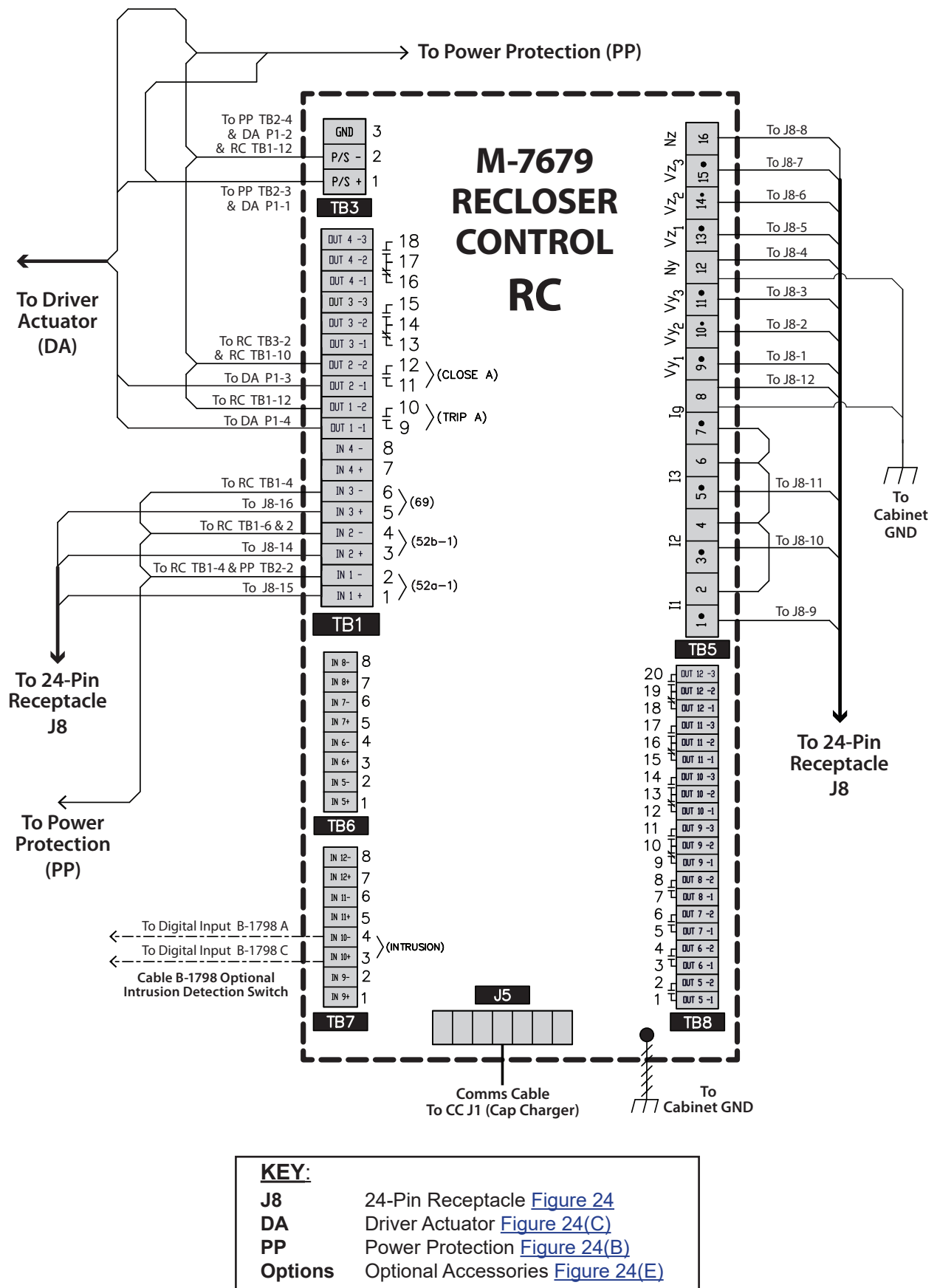
Figure 24(A) Cabinet Interface 24M – M-7679 (RC) Terminal Block Connections
