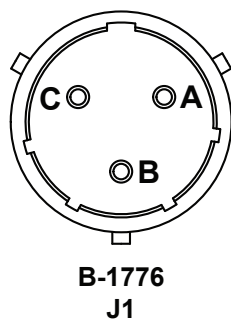
Figure 39 3-Pin Cannon AC Input Cable B-1776
