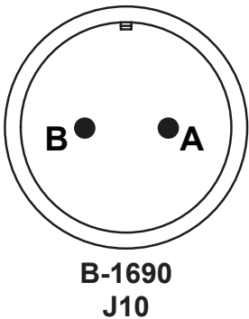
Figure 36 B-1690 2-Pin Cannon AC Input Cable
