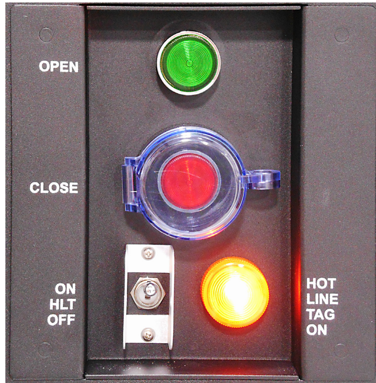
Figure 17 External Trip/Close with Hot Line Tag Assembly
