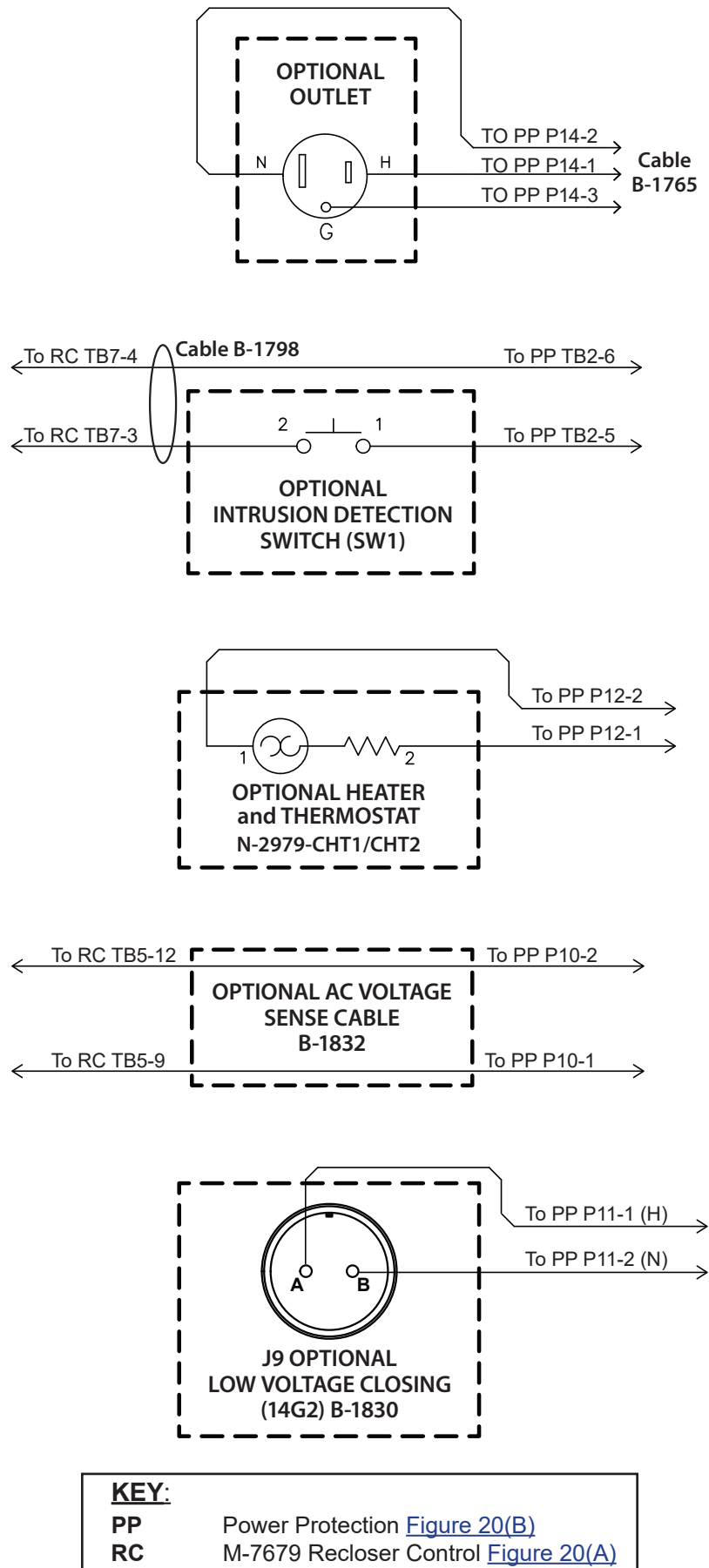
Figure 20(D) Cabinet Interface 14C2, 14G2 – Optional Accessories Connections
