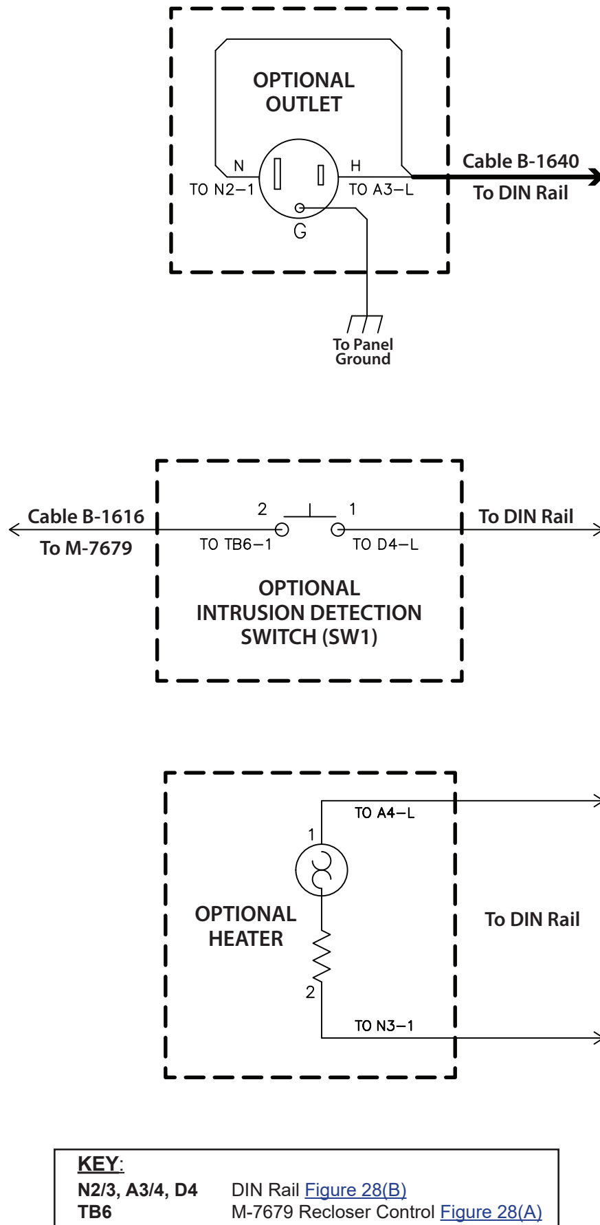
Figure 28(E) Cabinet Interface 42V – Optional Accessories Connections
