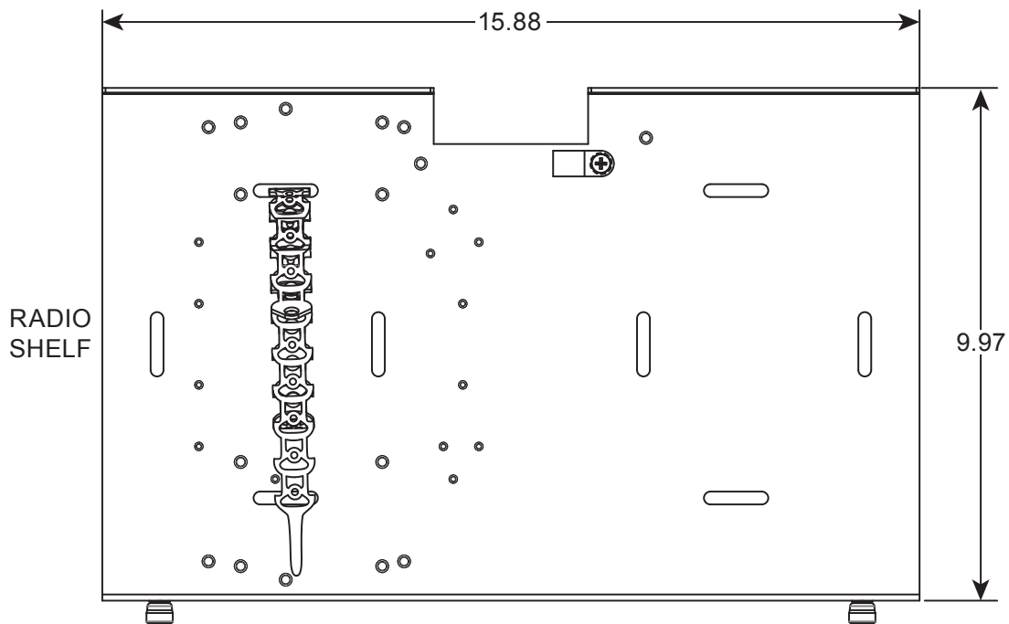
Figure 43 Universal Radio Shelf Dimensions
