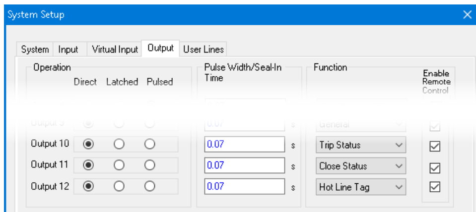
Figure 19 IPScom System Setup/Output Tab with Outputs 10, 11, and 12 Settings
