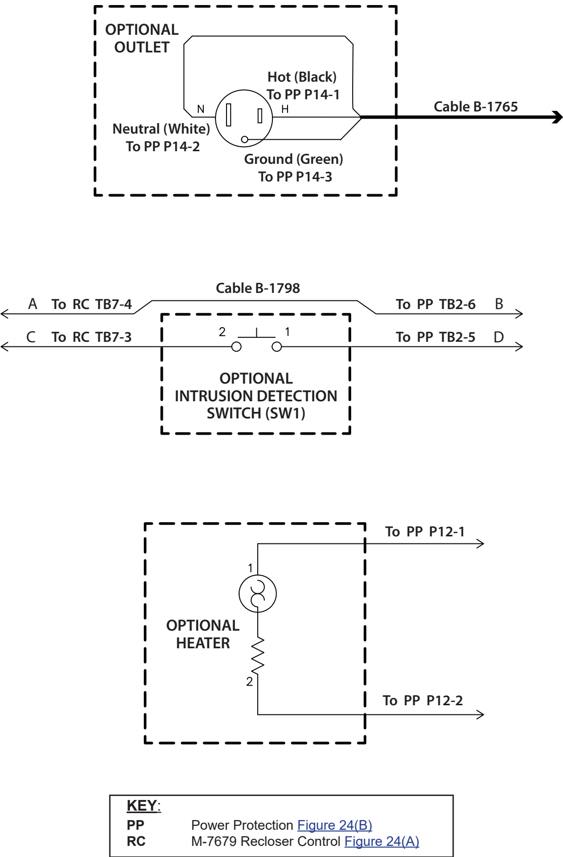
Figure 24(E) Cabinet Interface 24M – Optional Accessories Connections
