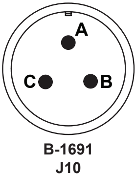
Figure 37 B-1691 3-Pin Cannon AC Input Cable
