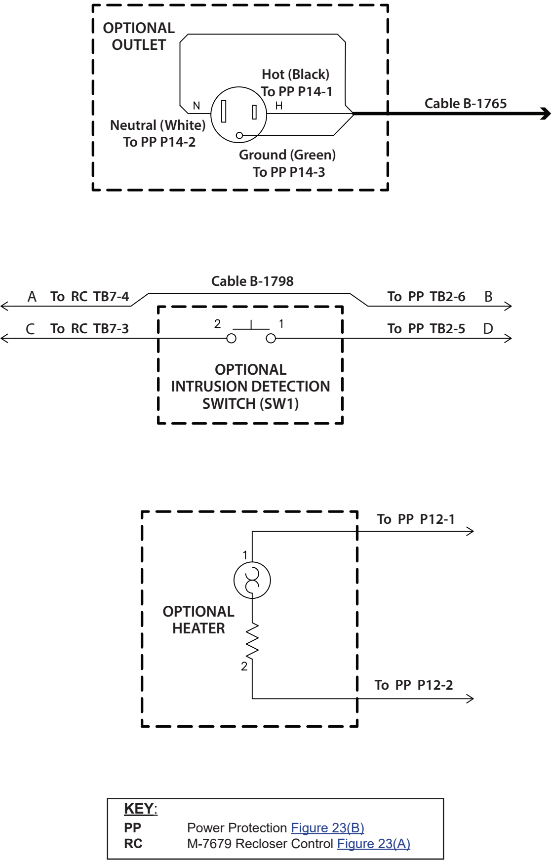
Figure 23(E) Cabinet Interface 24G – Optional Accessories Connections
