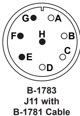
Figure 34 B-1783 with B-1781 Voltage Sensing Cable
